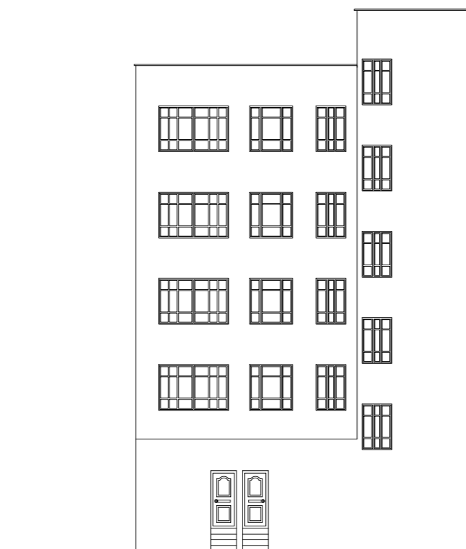
WEST ELEVATION Scale 1:100
